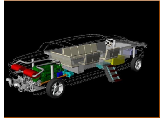
Nouvoyage Limousine Tender 33', Ghost View
